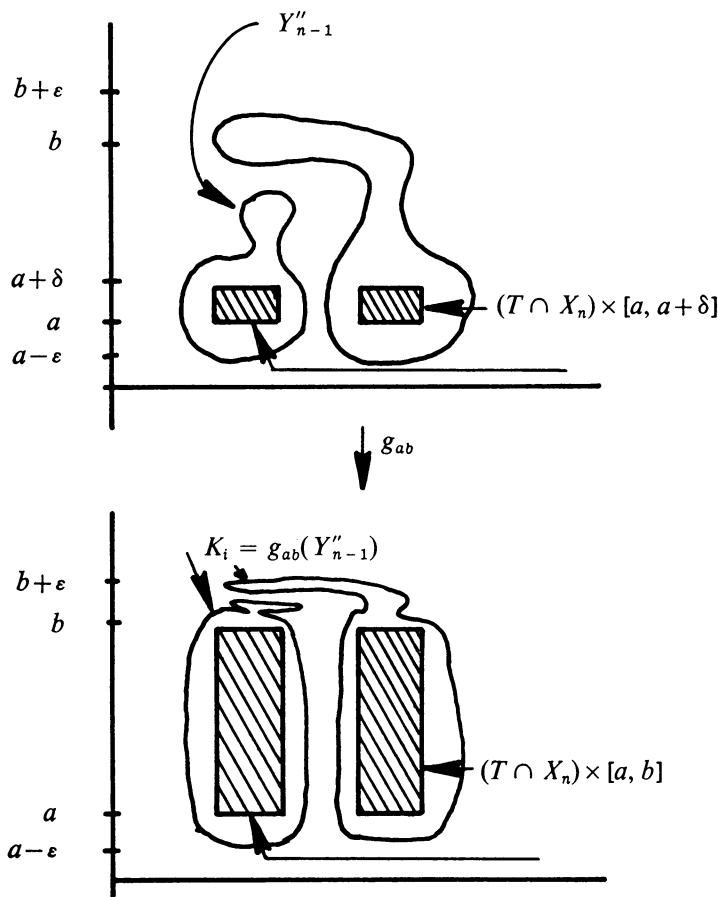
FIGURE 5. Expanding 4-cells
